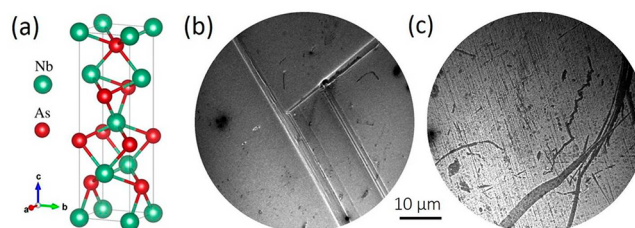
Figure 1. (a) Molecular structure of NbAs. (b) MEM at start voltage ( V_{\text{st}} = -0.25 V). (c) MEM at V_{\text{st}} = -0.56 V.
